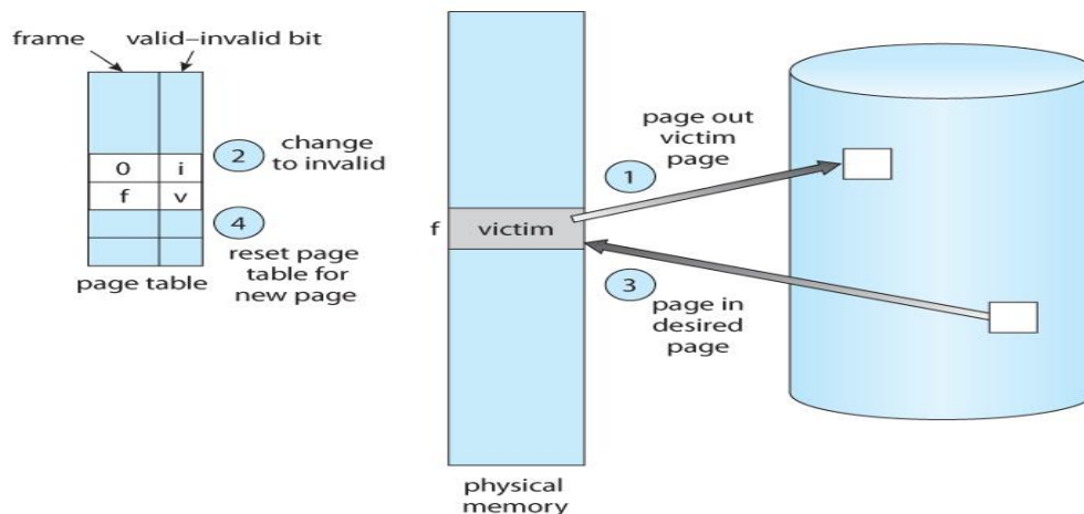
Figure 4.32 - Page replacement.
